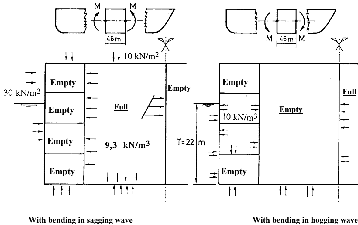
Figure 6 - Considered loading cases.
