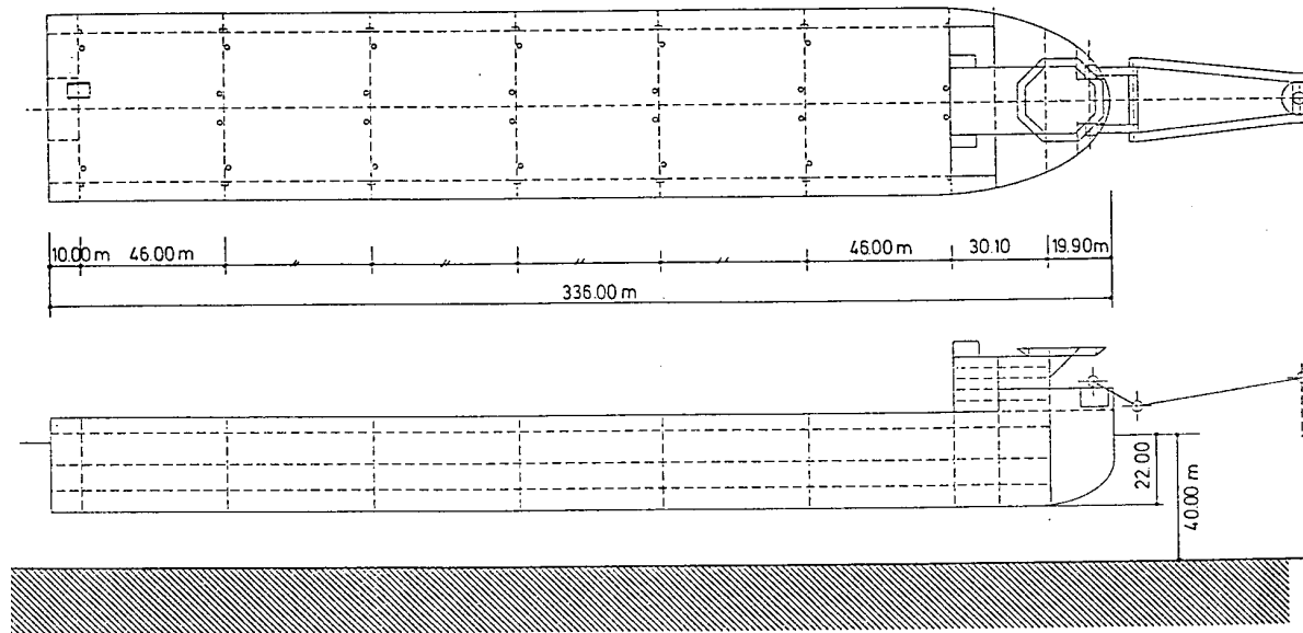
Figure 5 - General view of the FSO barge
