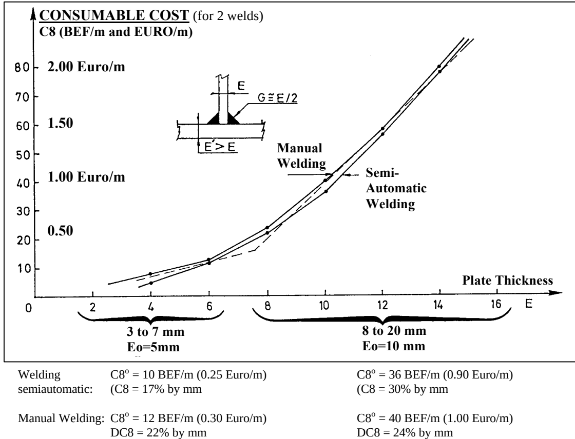
Figure 3 - Consumable Costs for 1 m of Welding of a Stiffener (two welds).
