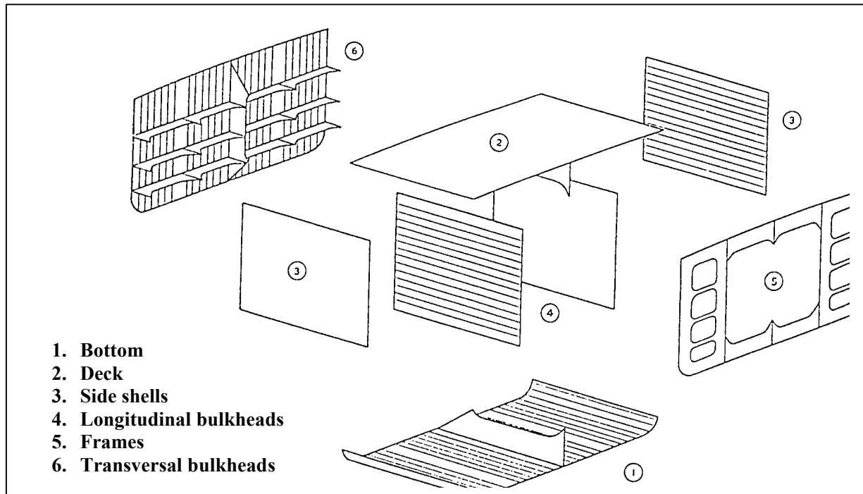
Figure 2- Subdivision of a Block into Elements (Buxton 1966)
